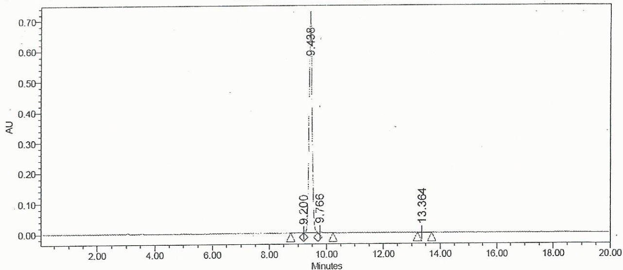
Auto-Scaled Chromatogram
